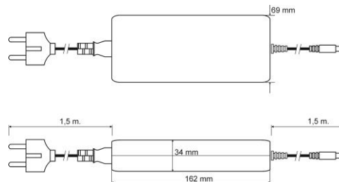
Fig.1. Dimension of power supply.
